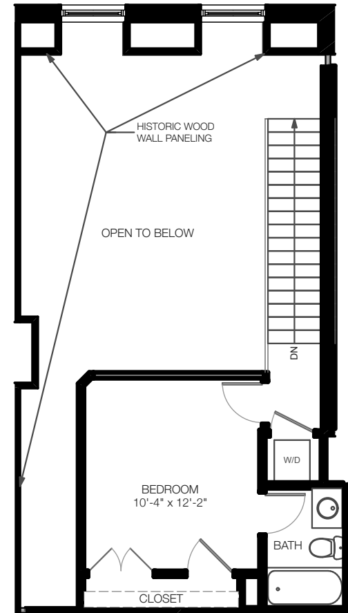
UPPER LEVEL
